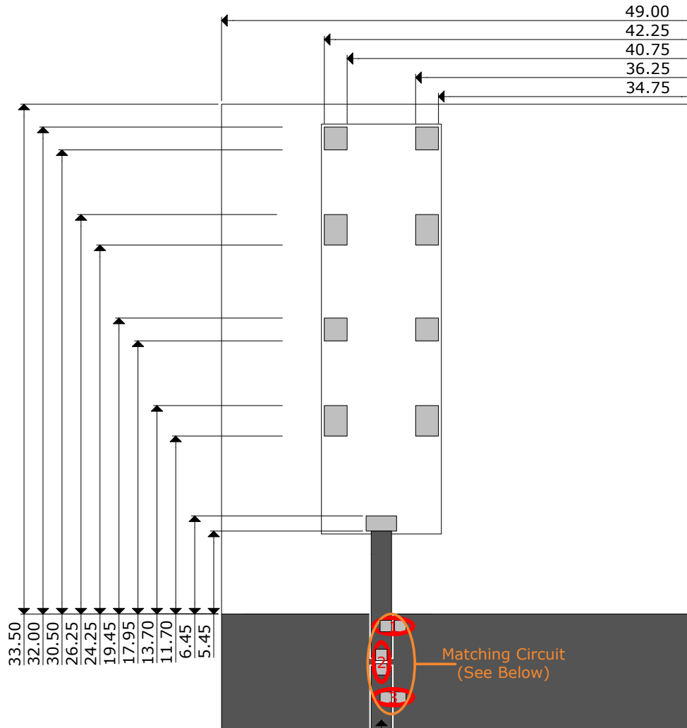
Transmission Line With 50Ω Impedance Characteristics
