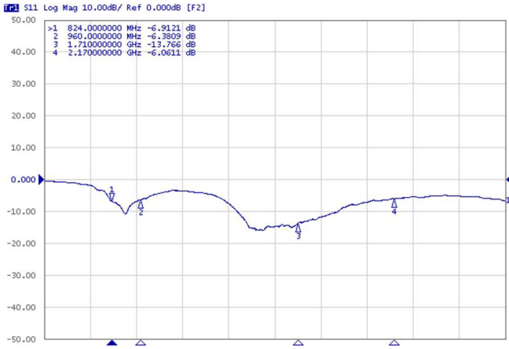
Return Loss
