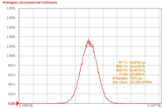
Frequency - 212.500MHz
