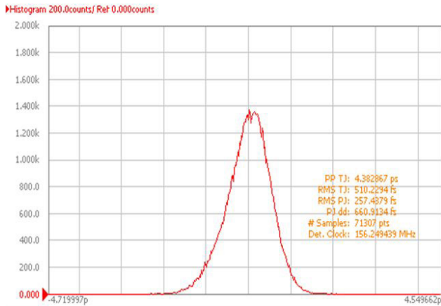
Frequency - 156.250MHz
