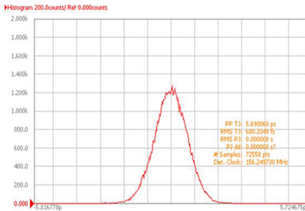
Frequency - 156.250MHz
