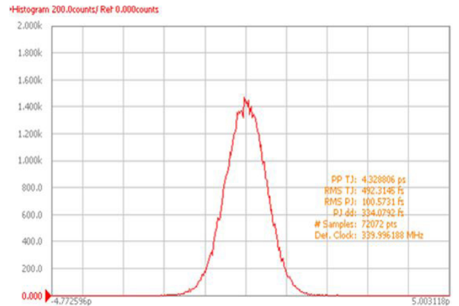
Frequency - 340.000MHz
