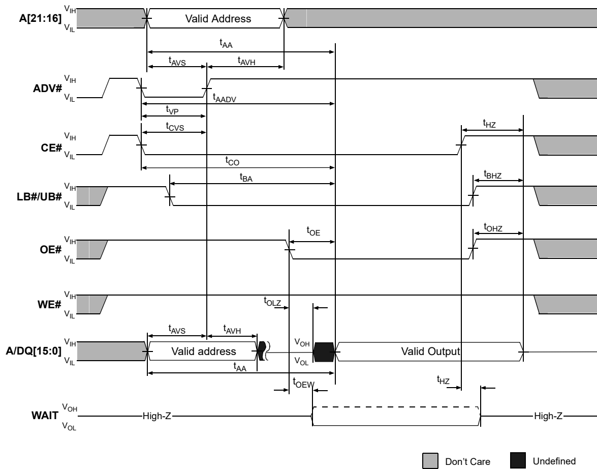
Figure 24: Asynchronous READ
