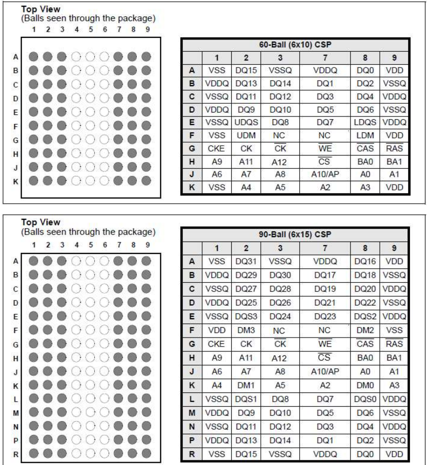
Figure 1.1 - PIN DESCRIPTION
