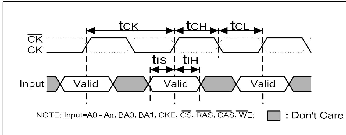
Figure 6 - Basic Timing Parameters
