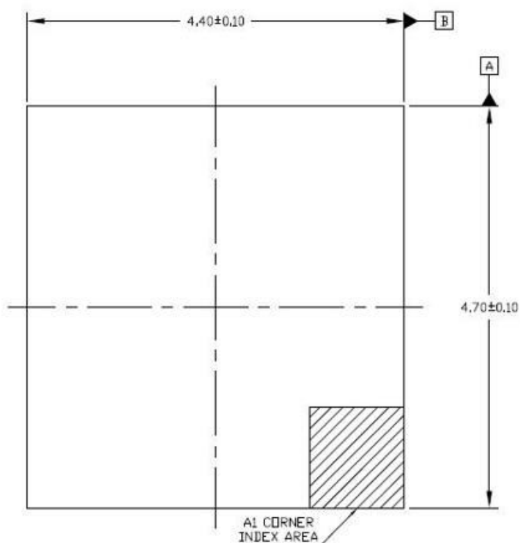
TOP VIEW
