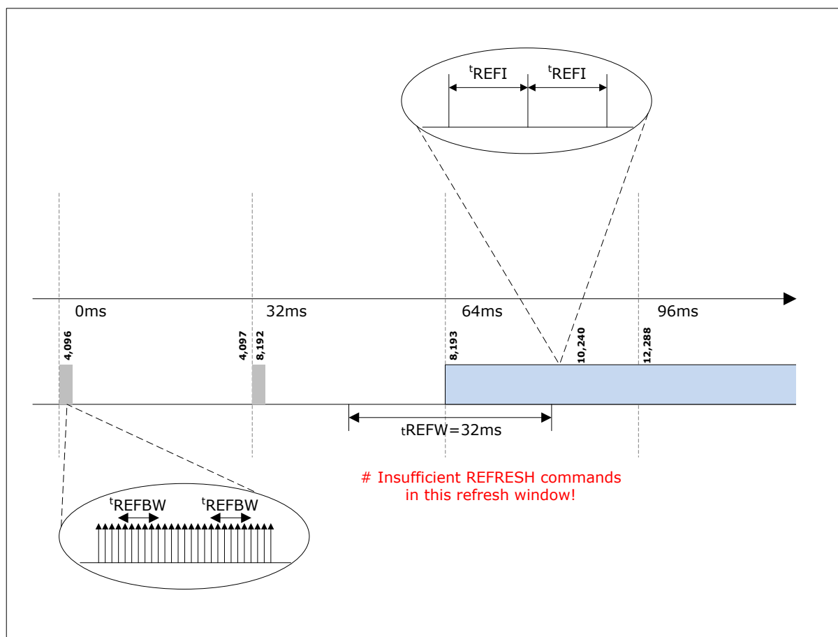
Figure 4.29 - NOT-Allowable Transition from Repetitive Burst Refresh with Subsequent Refresh Pause to Regular, Distributed Refresh Pattern
