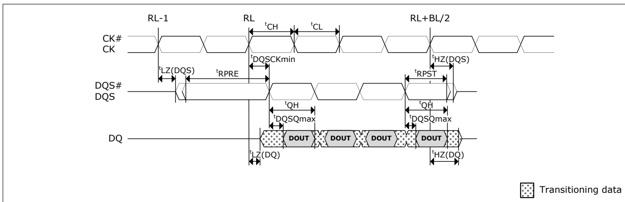
Figure 4.5 - Data output (read) timing (tDQSCKmin)
