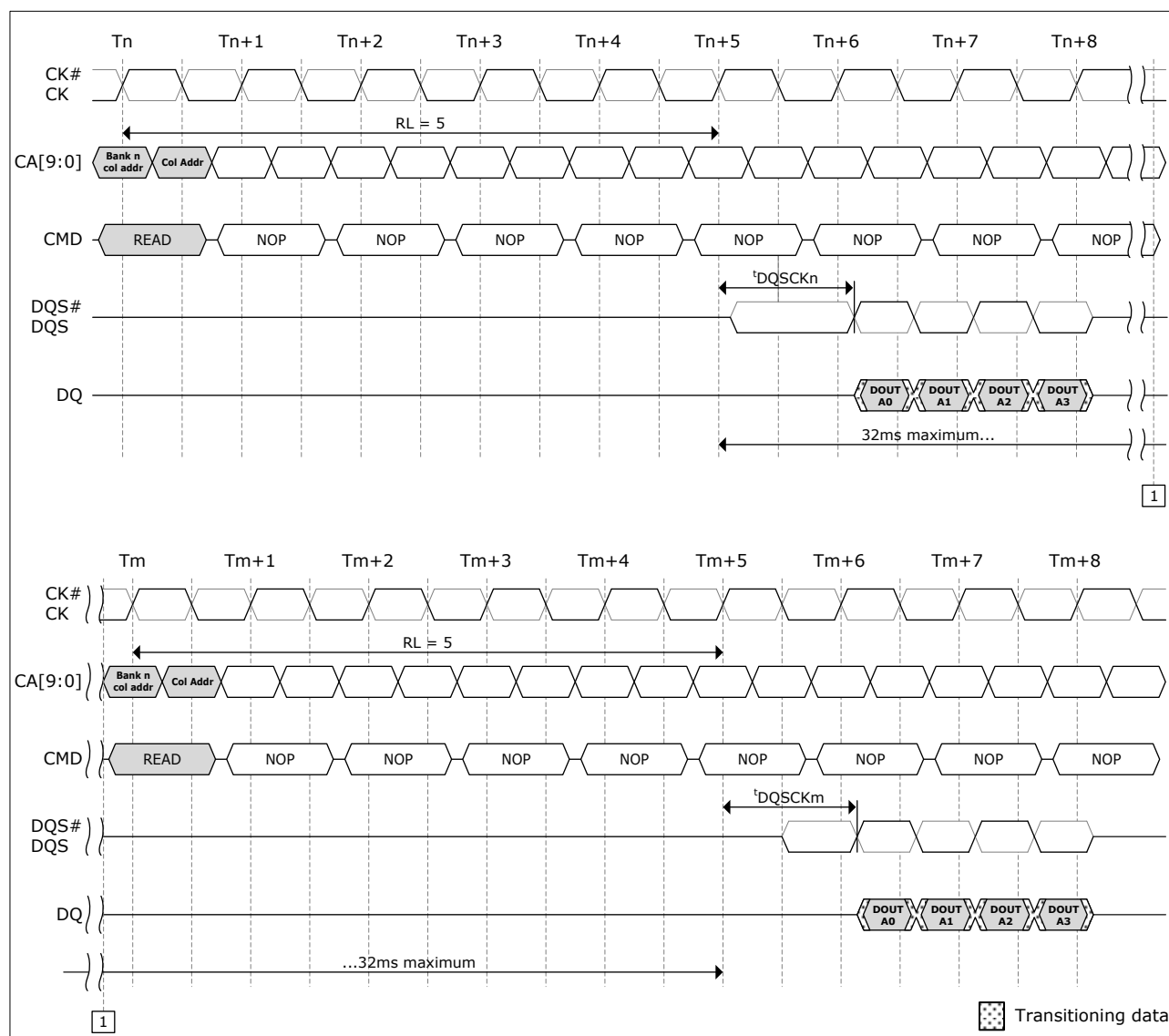
Figure 4.8 - t_{DQCKDL} timing
