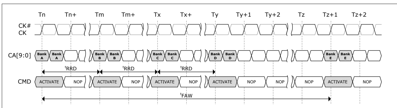
Figure 4.2 - t_{FAW} timing
