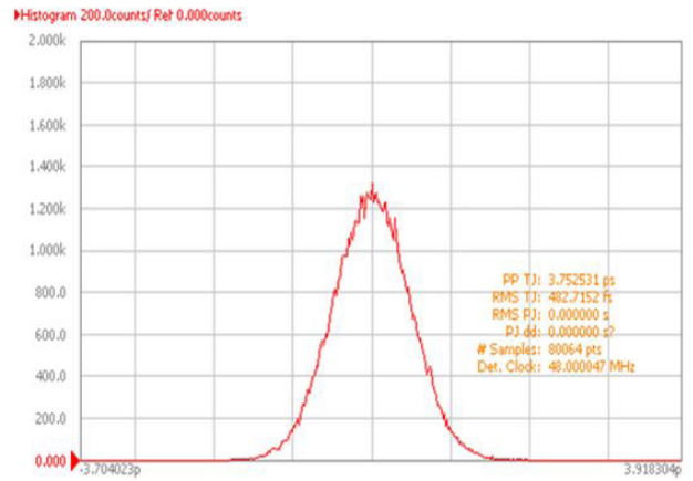
Frequency - 48.000MHz
